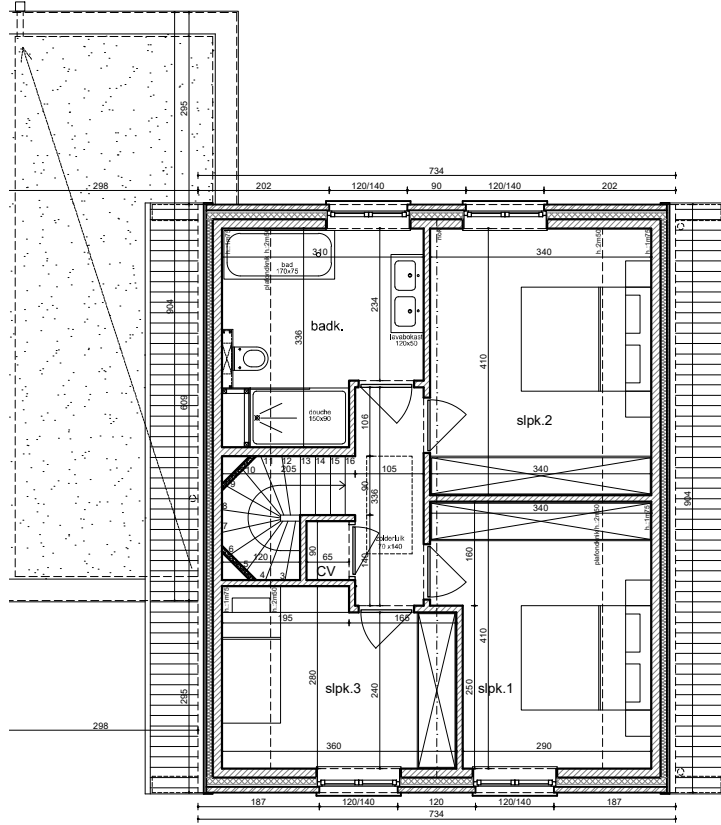
LOT 27 - VERDIEPING
