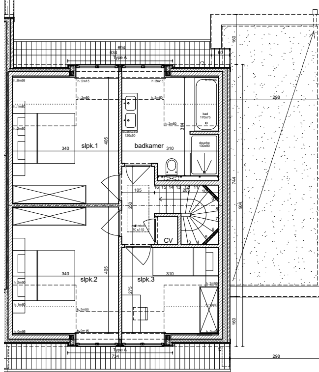
LOT 28 - VERDIEPING
